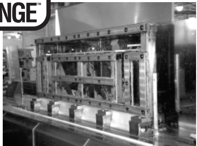
Ball Lock Angle Fixture for Larger Applications
