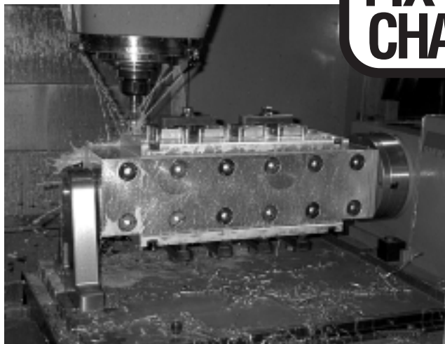
SMW Indexer With Horizontal Ball Lock Column
