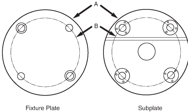
Fixture Plate
